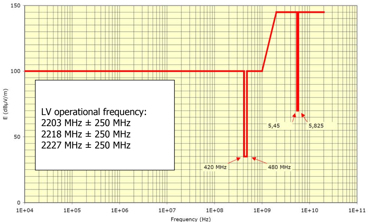
Figure 4.2 – LV susceptibility level at spacecraft/adaptor interface
