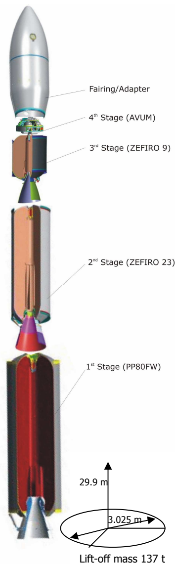
Figure 1.1 – LV property data
