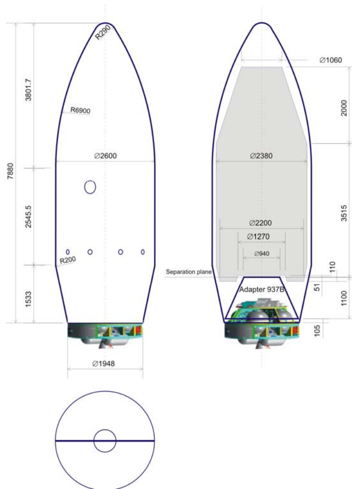
Figure 5-3 – Fairing external dimensions and payload volume
