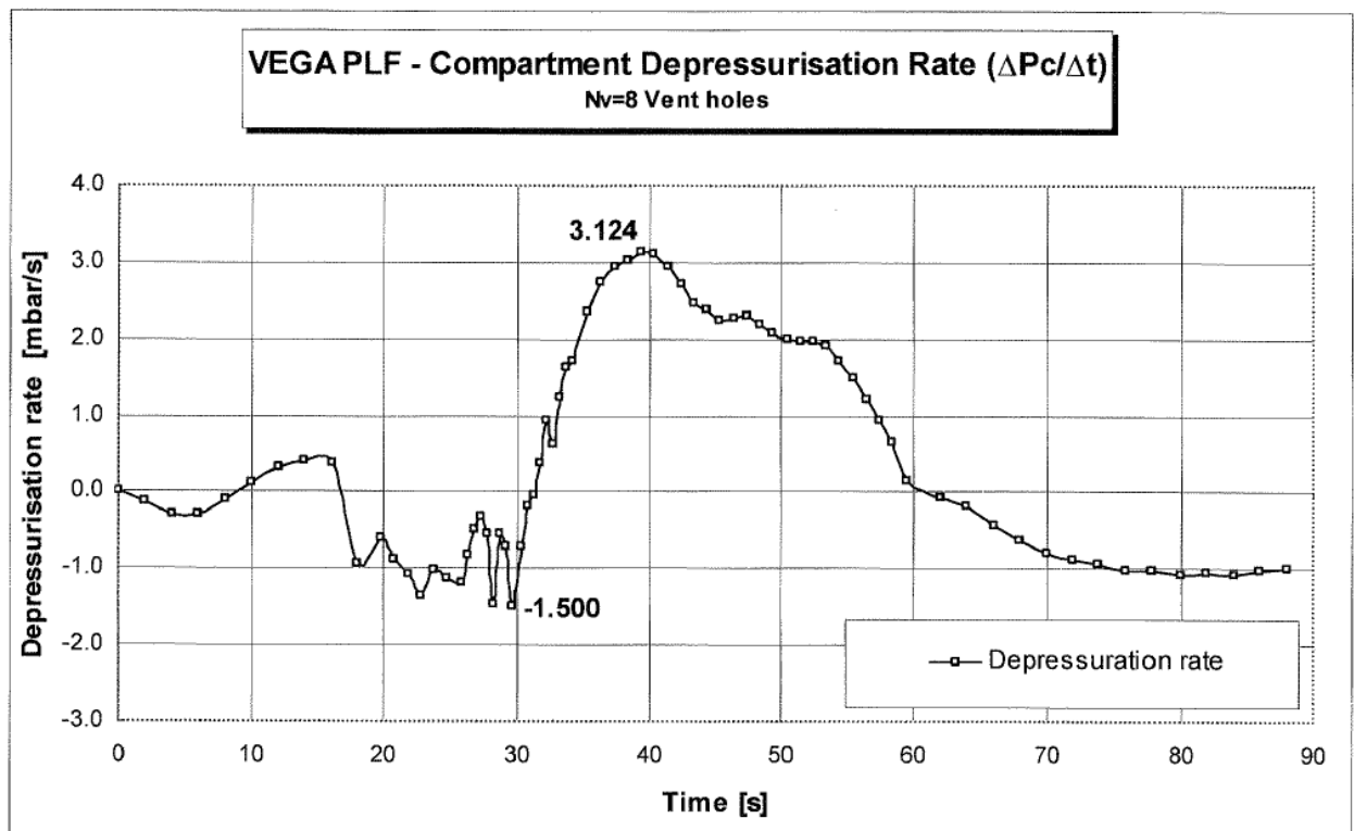
Figure 3.6 - The evolution of the compartment depressurization rate
