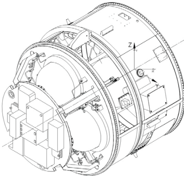
Figure A5- 7 : AVUM stage in shipment configuration (Integrated with 3TAvm inter-stage)
