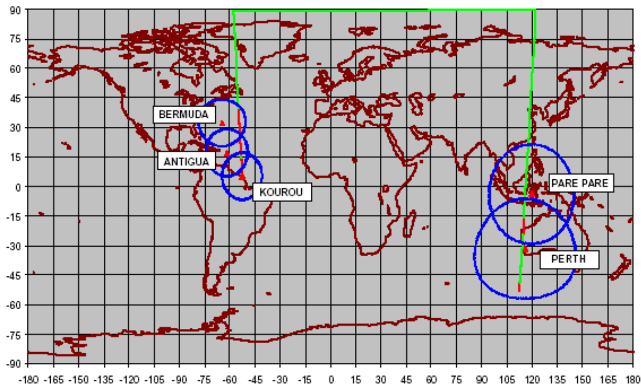
Figure 2.2 – Typical ground path for the Vega reference mission
