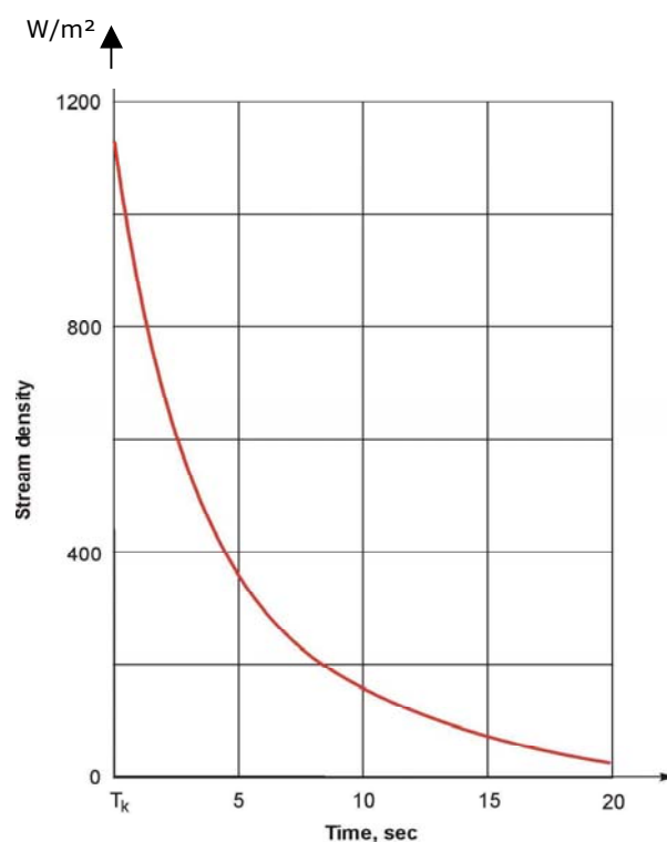
Figure 3.3 – Typical Aerothermal Flux Decay after fairing jettisoning
