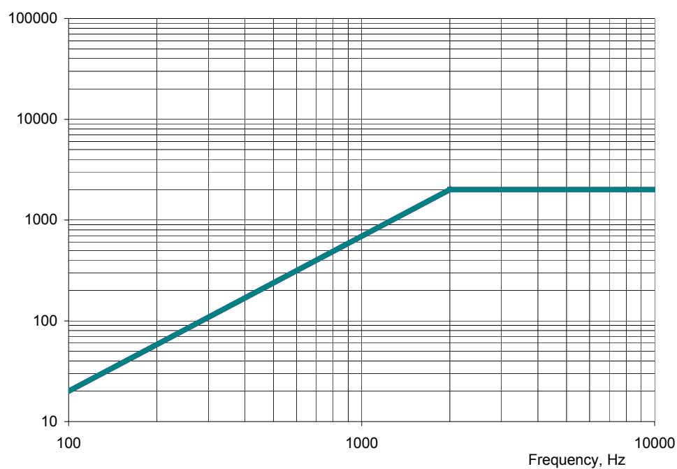
Figure 3.4 - The envelope acceleration shock response spectrum (SRS) at the spacecraft base
