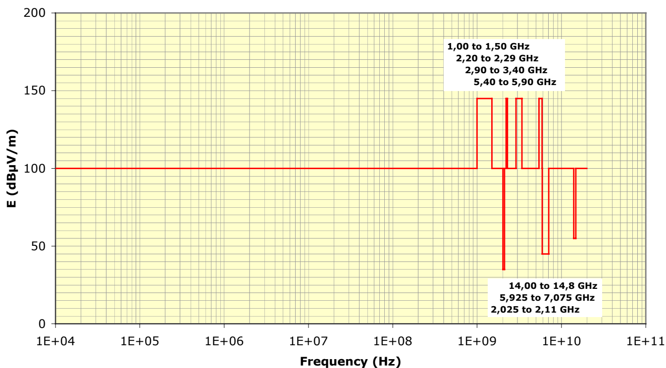
Figure 3.4 - Intensity of electrical field generated by spurious or intentional emission from the launch vehicle and the range
