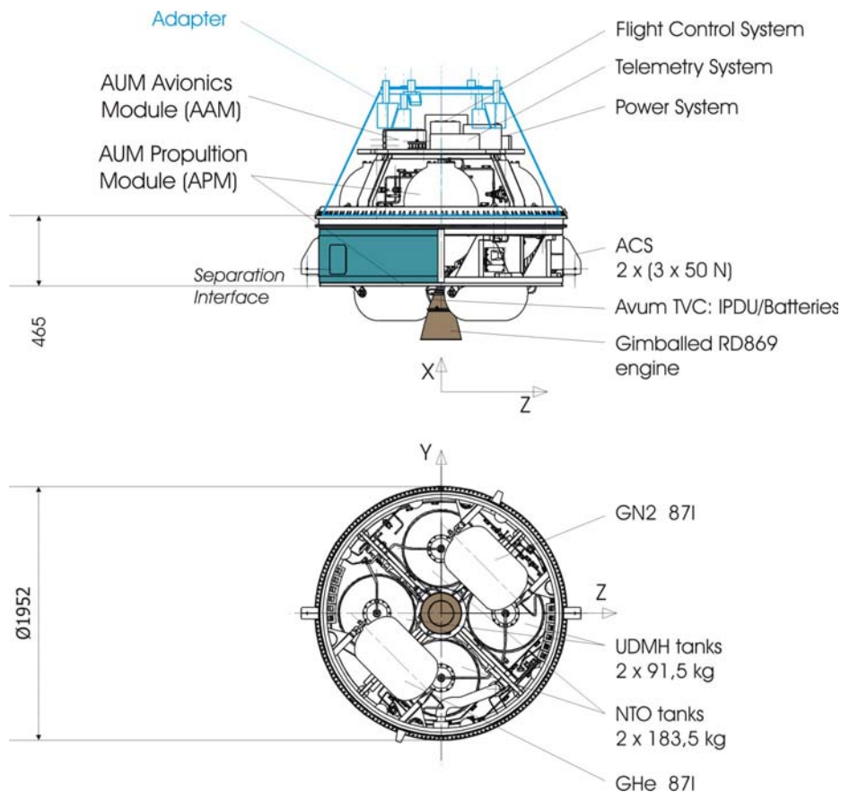
Figure A5- 5 : 3rd Stage Layout
