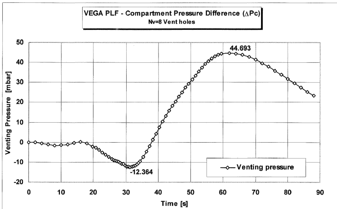
Figure 3.5 - The evolution of the compartment differential pressure
