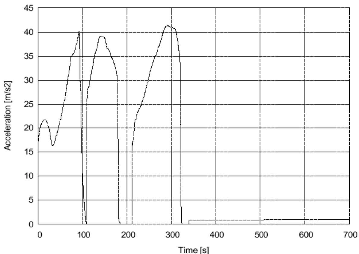
Figure 3.1 – Typical Longitudinal Steady-state Static Acceleration for the reference mission.
